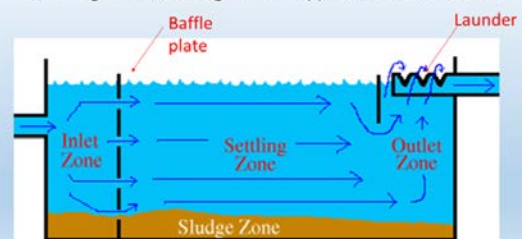
Rectangular Settling Tank - typical cross section
